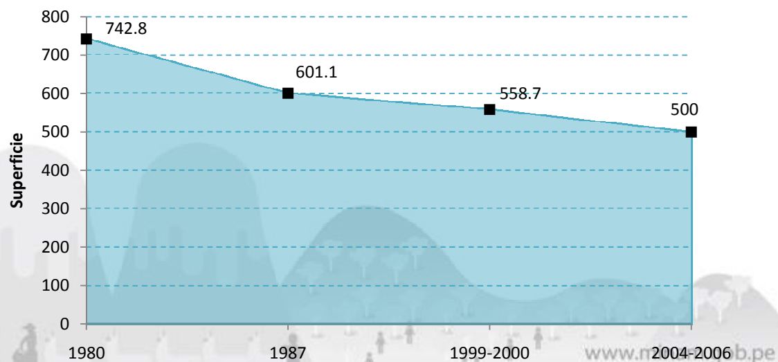
CORDILLERA BLANCA GLACIER COVERAGE (KM 2 )
