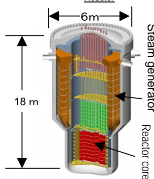
Small and Medium Reactor
