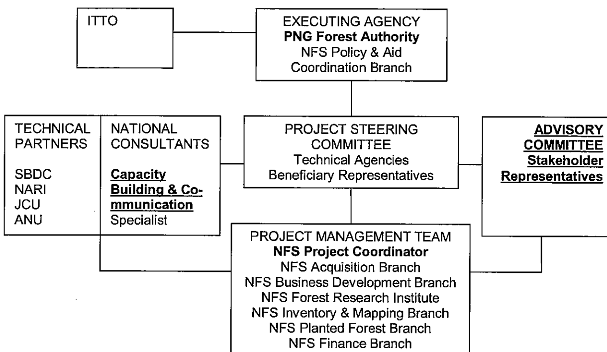
Figure 6: Project Structure
