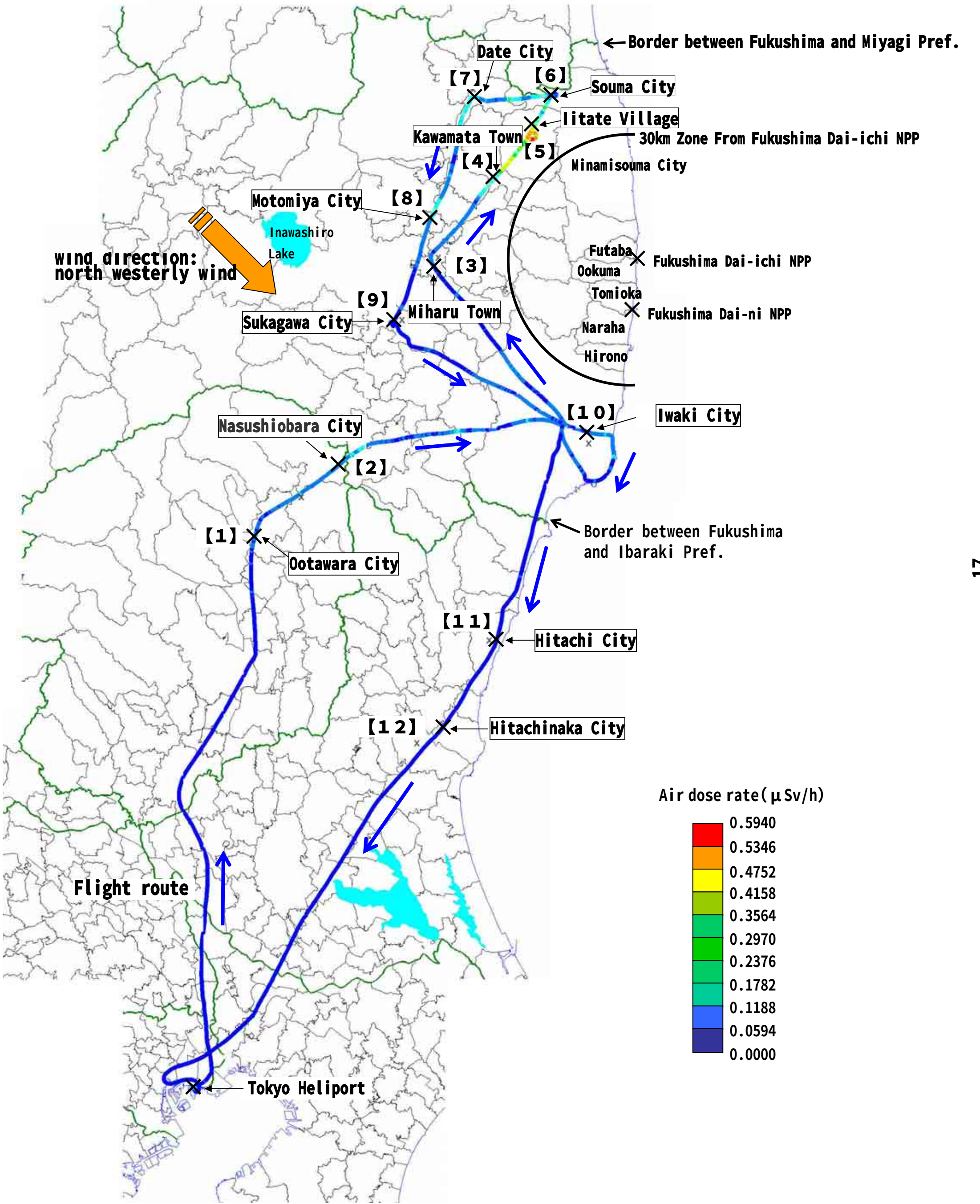
Flight route of helicopter monitoring on April 12, out of Fukushima Dai-ichi NPP ([1] ~ [12] : Major Monitoring Point)
