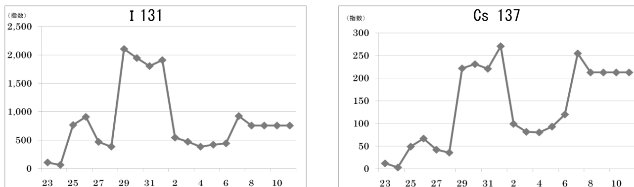
[Figure 1] Scenario of Radioactivity Concentrations in the Effluent Discharged from the Fukushima Dai-ichi NPP
